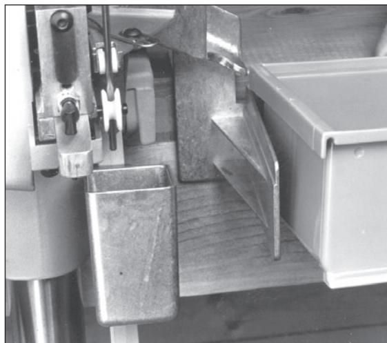
Fig. 3 - The cartridge collection bin (#13839) simply slides onto the bracket and will be in the proper position.
